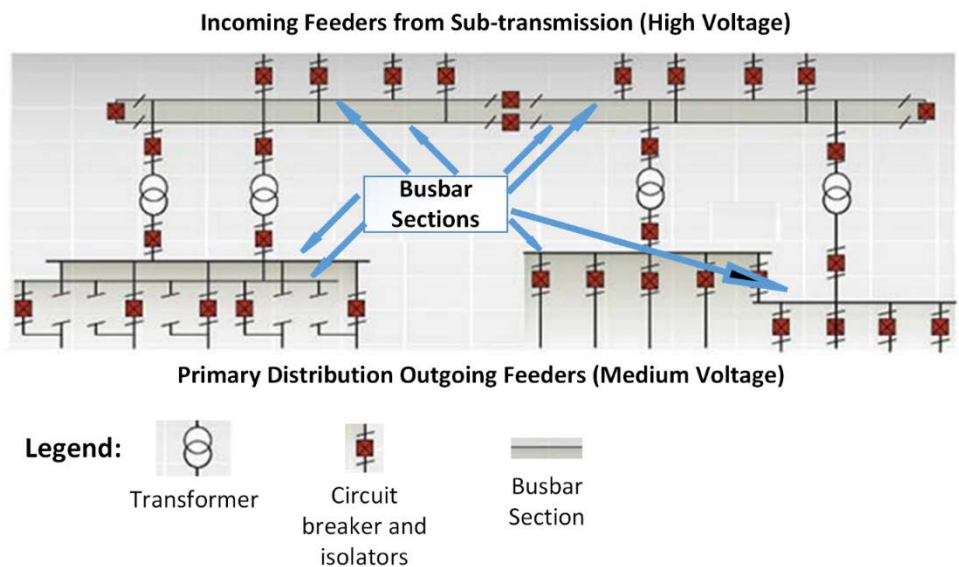
Figure 2: A typical load area substation single line diagram showing its major components.
