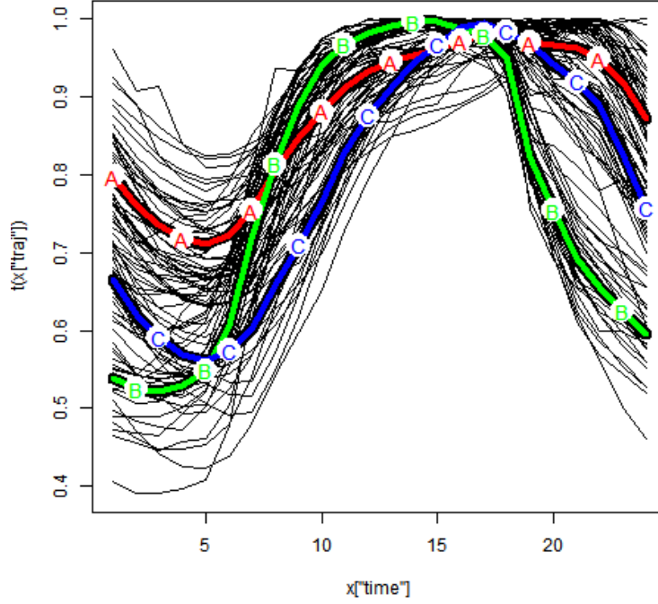
Figure E-2: Hourly Load Trajectories and Clusters
